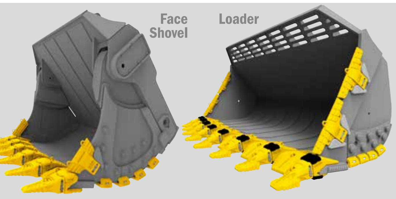
CAST CORNER
